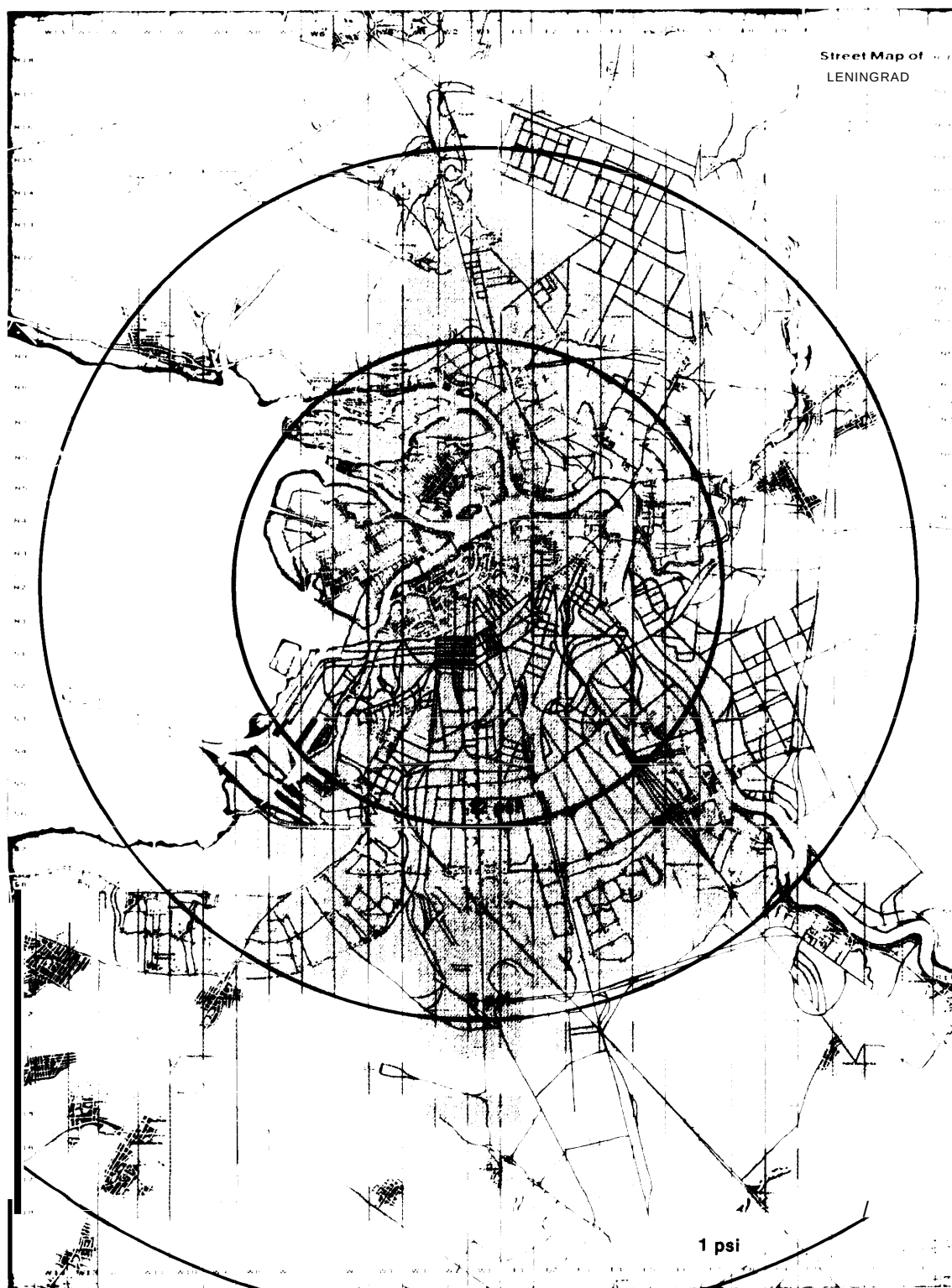
Figure 11.—Leningrad 9-Mt Air Burst
