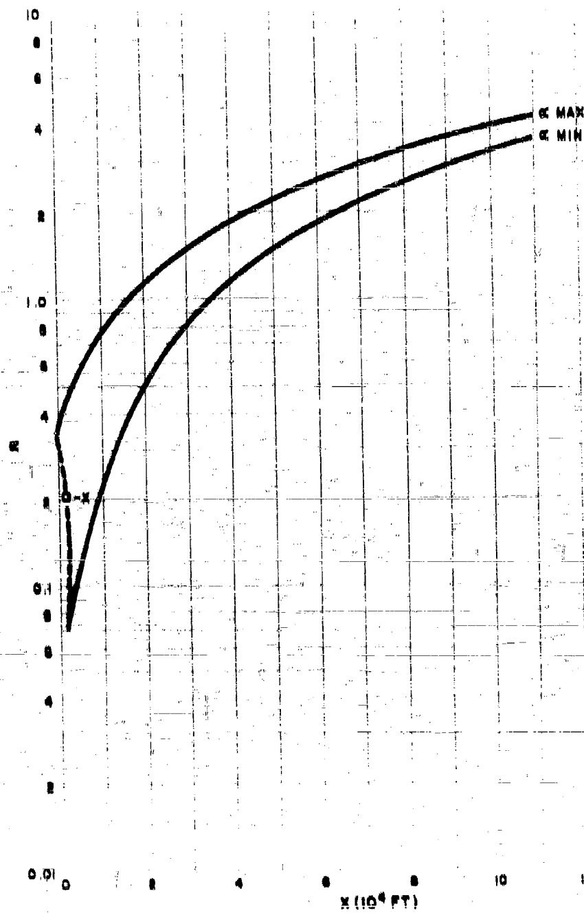
Figure 5.10 VARIATION OF \alpha_{(10)} AND \alpha_{(10)} WITH DOWNWIND DISTANCE FOR A 1-MT YIELD SURFACE DETONATION AND WIND SPEED OF 15 MPH
