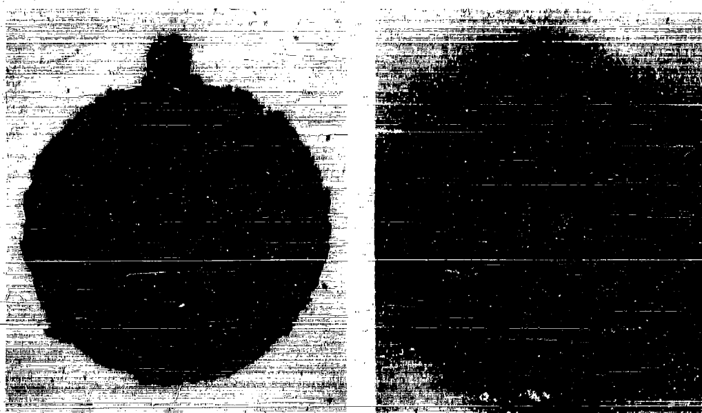
Figure 2.9 THIN SECTION AND RADIOGRAPH OF A FALLOUT PARTICLE FROM A MODERATE-YIELD TOWER SHOT AT THE ENIWETOK PROVING GROUND. THIS PARTICLE IS COMPOSED ENTIRELY OF MAGNETITE AND THE RADIOACTIVITY IS DISTRIBUTED UNIFORMLY THROUGHOUT ITS VOLUME
