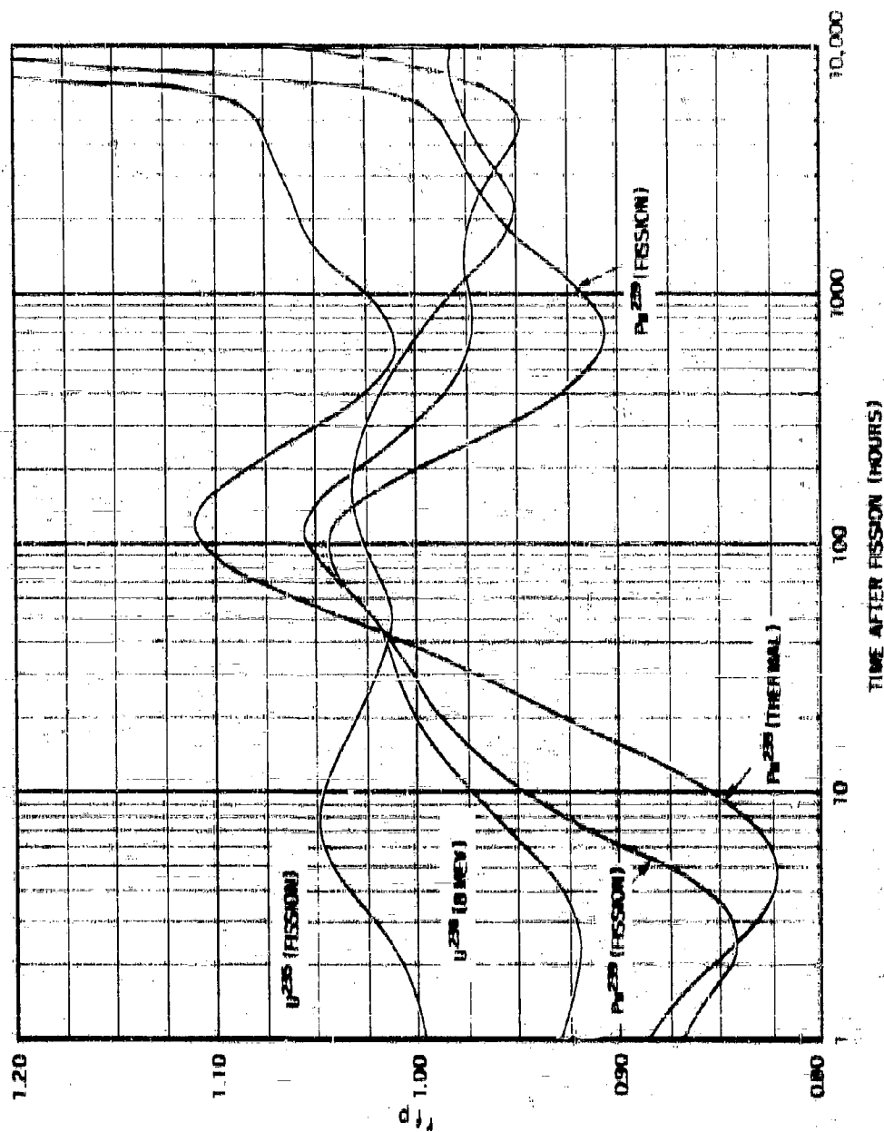
Figure 3.5 GROSS AIR IONIZATION RATE FRACTIONATION NUMBER, r_{\text{eff}} , RELATIVE TO THE IONIZATION RATE (in \mu\text{meters} ) OF THE FISSION PRODUCTS FROM THERMAL NEUTRON FISSION OF U-235. FOR THE FISSION PRODUCT MIXTURES FROM OTHER FISSION NUCLEIDES AND NEUTRON ENERGIES
