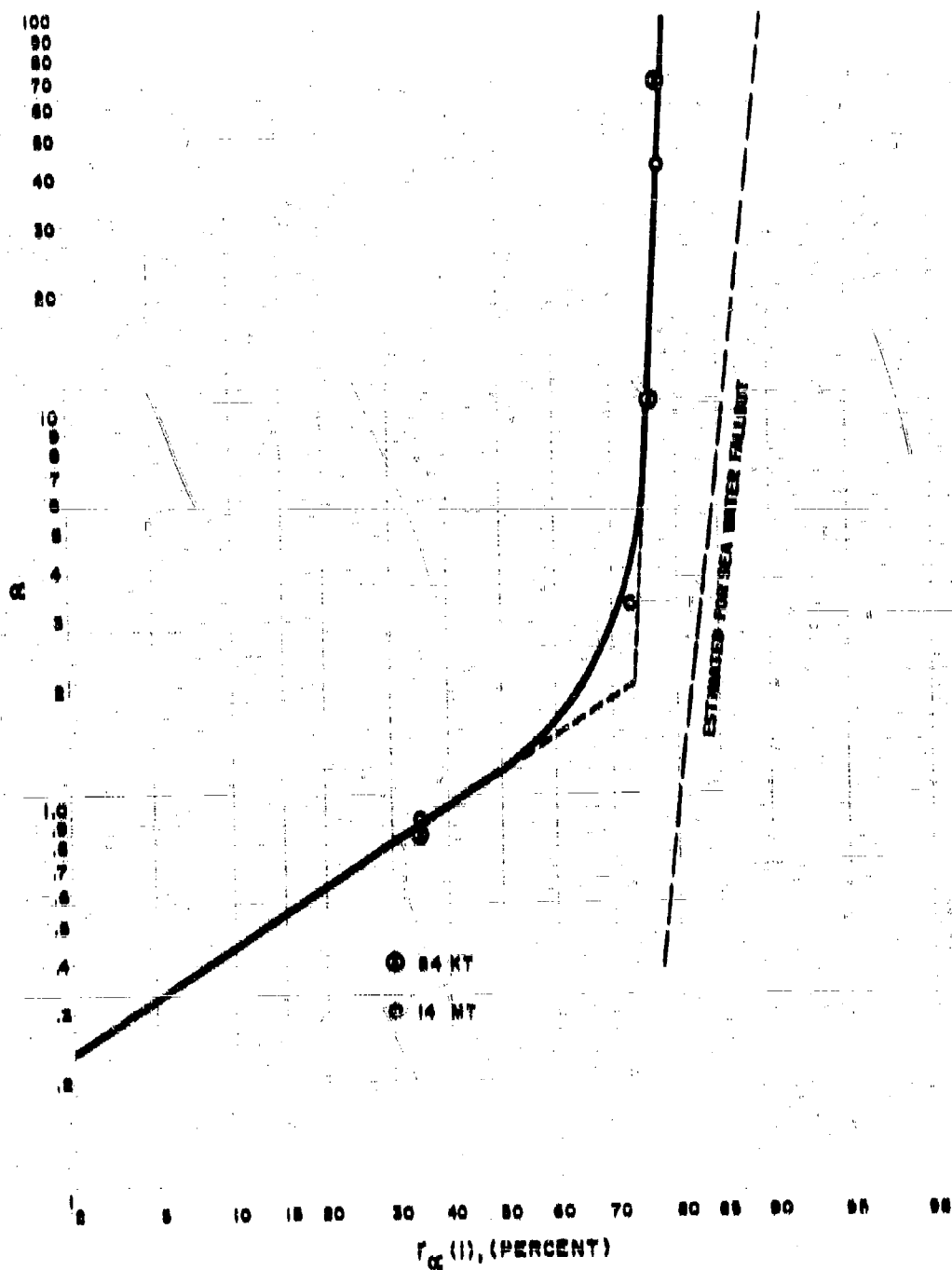
Figure 6.2 ESTIMATED PERCENT OF THE FISSION PRODUCT ACTIVITY IN r_{\alpha} AT 1 HR FROM THE FISSION PRODUCTS CONDENSED ON PARTICLE GROUPS WITH r_{\alpha} VALUES (15 MPH Wind Speed) LESS THAN A STATED VALUE
