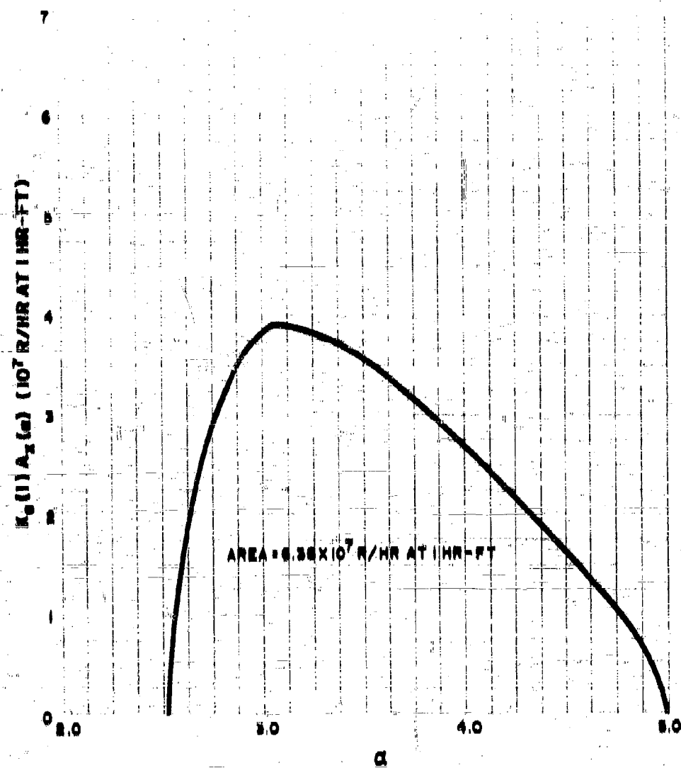
Figure 8.5 VARIATION OF K_0(1)A_z(\alpha) WITH \alpha AT x = 1.87 \times 10^5 FT FOR W = 10^3 KT AND A WIND SPEED OF 15 MPH
