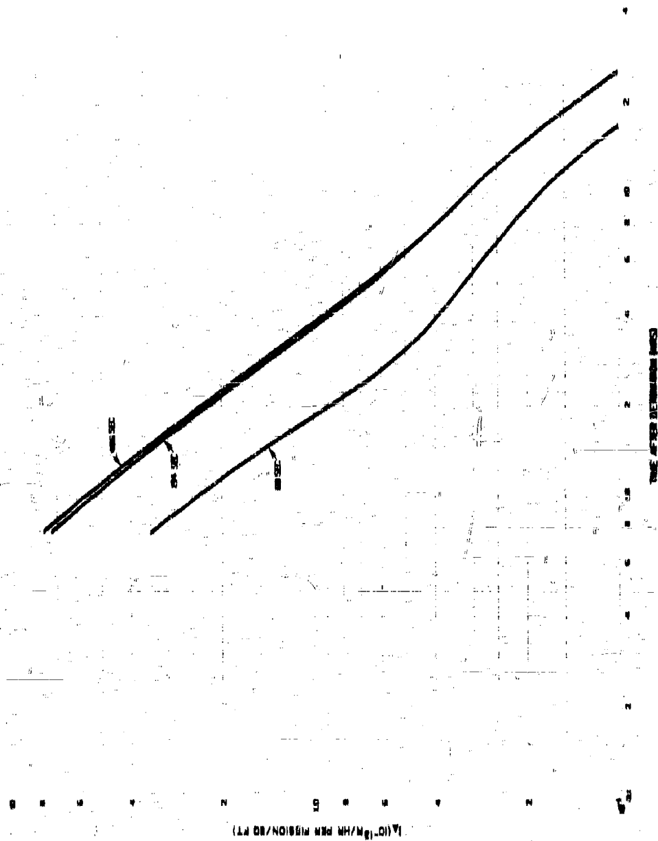
Figure 6.3 CALCULATED IONIZATION RATE AS A FUNCTION OF TIME AFTER DETONATION FOR ASSUMED CONDENSATIONS UP TO 60, 174, AND 436 SECONDS AFTER FISSION OF FISSION PRODUCTS FROM 2-MG NEUTRON FISSION OF U-235 AND AN ASSUMED SURFACE BURST TOTAL YIELD OF 14-KT
