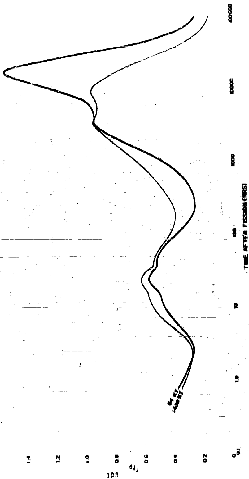
Figure 3.10 VARIATION OF \bar{\nu}_e WITH TIME AFTER FISSION FOR THE FRACTIONATED MIXTURE OF FISSION PRODUCTS FROM ^{235}\text{U} NEUTRON FISSION OF U-235
