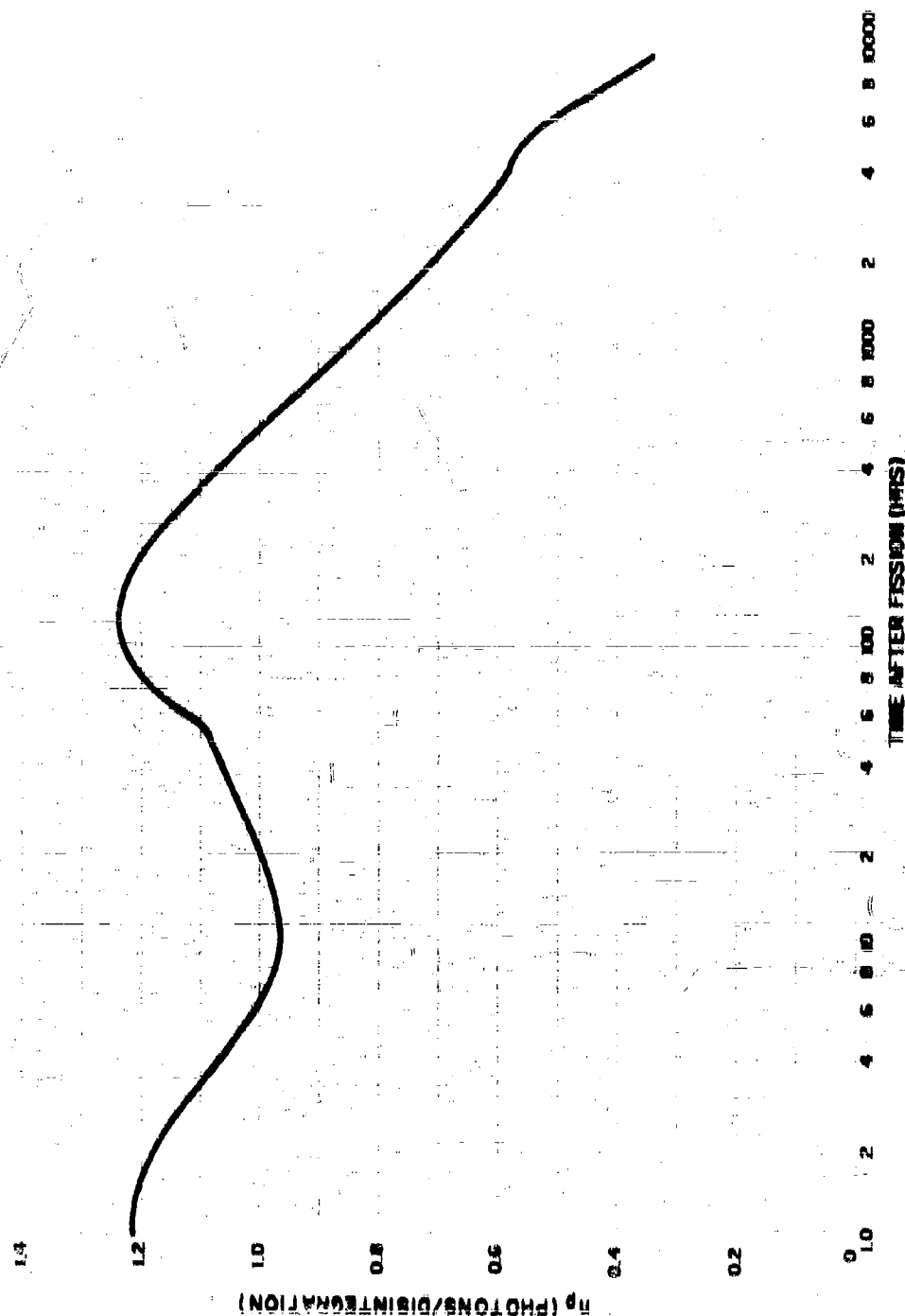
Figure 3.7 NUMBER OF PHOTONS PER DISINTEGRATION FOR THE NORMAL MIXTURE OF FISSION PRODUCTS FROM 0.4% NEUTRON FISSION OF U-235
