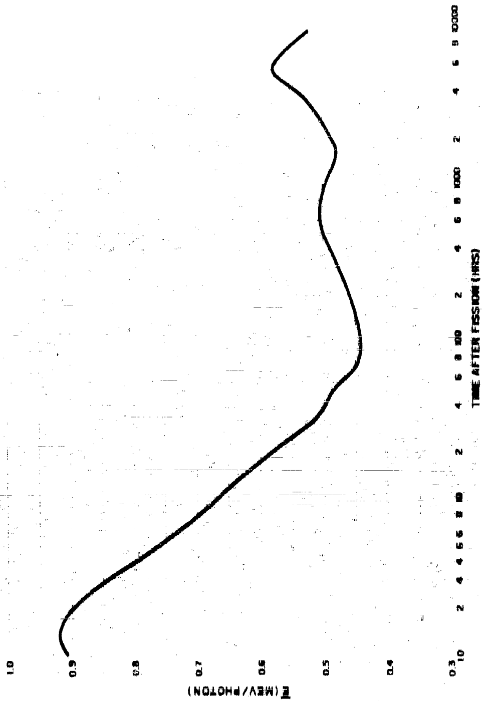
Figure 3.8 AVERAGE ENERGY OF THE PHOTONS FROM THE NORMAL MIXTURE OF FISSION PRODUCTS FROM B-46- NEUTRON FISSION OF U-238
