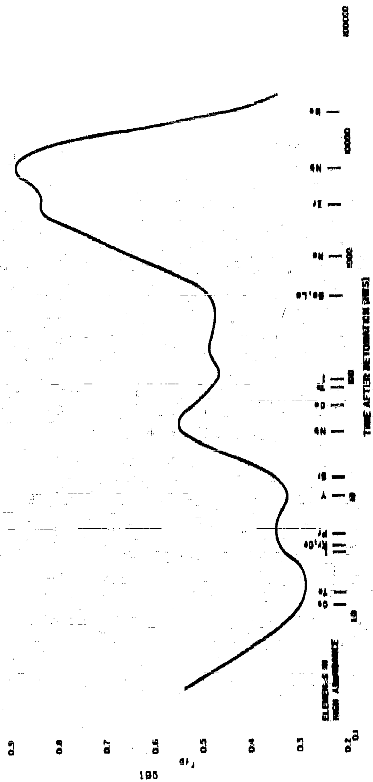
Figure 3.11 OBSERVED VARIATION OF \tau_{\text{eff}} WITH TIME AFTER FISSION FOR CLOSE-IN FALL-OUT FROM A LOW TOWER SHOT AT THE NEVADA TEST SITE
